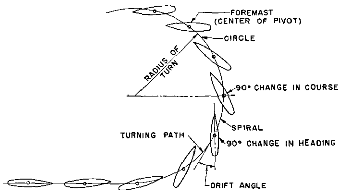
FIGURE. 160.—Successive positions of ship making 180^\circ turn.
