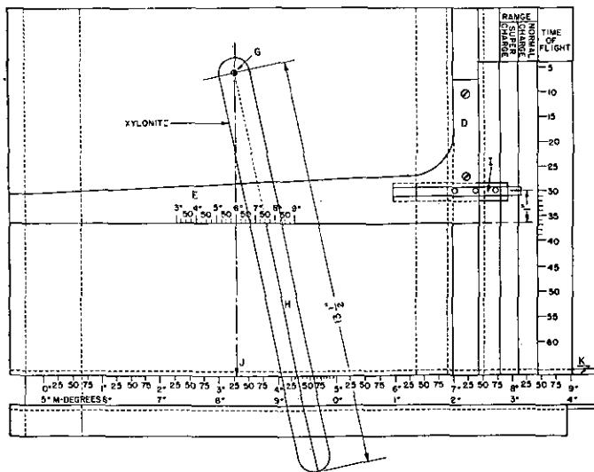
FIGURE 76.—Angular travel computer.
