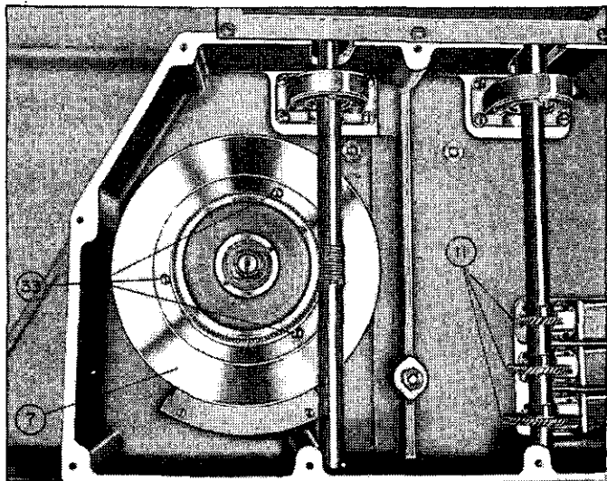
7. Azimuth scale. 11. Three spiral gears. 33. Screws holding azimuth scale.
