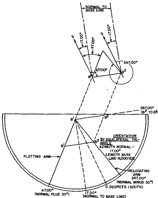
FIGURE 66.—Orientation of M1923 board (also M1)—equilateral triangle method.
